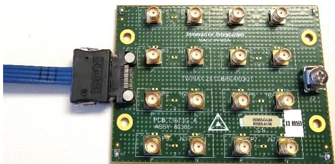
Figure 15. 80365-4 Breakout Board
