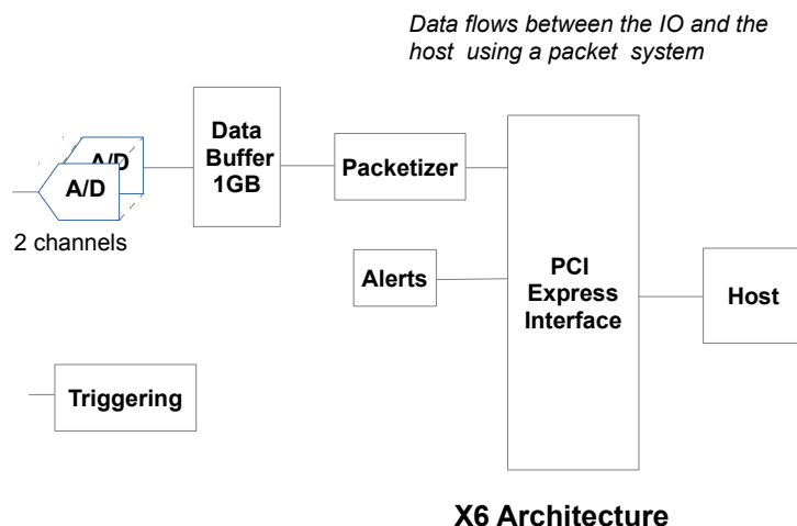
X6 Architecture
