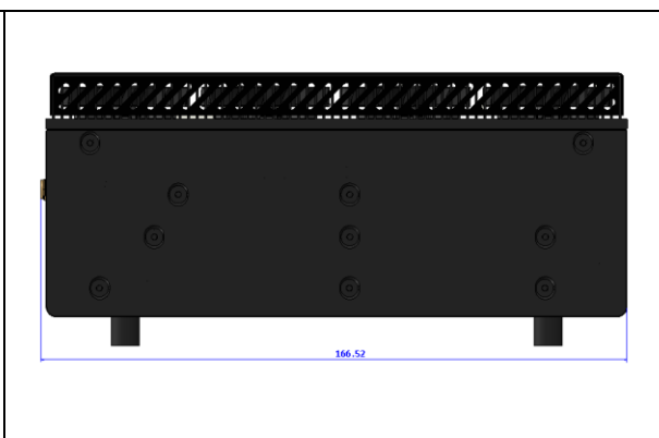
Figure 9. Nominal dimensions of the SBC-Nano chassis, side view.
