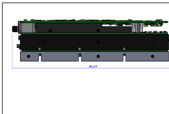
Figure 8. Nominal dimensions of SBC-Nano electronics stack, side view.
