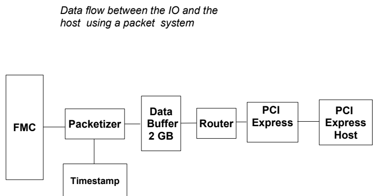
Example PEX7-COP Architecture
