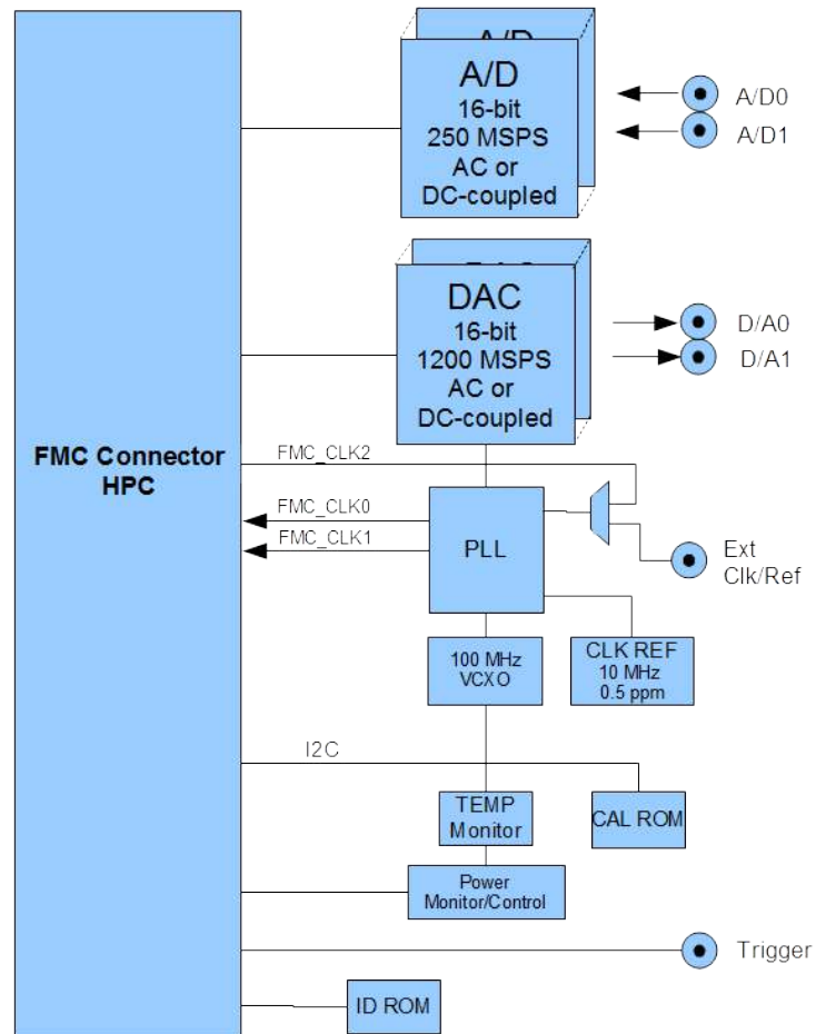
FMC-250 Block Diagram
