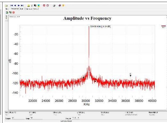
20-40 MHz Zoom into AC-Coupled A/D channel 0 wideband signal quality, F_{in} = 30.5 MHz through 7-pole TTE filter, F_s = 250 MHz onboard PLL.
