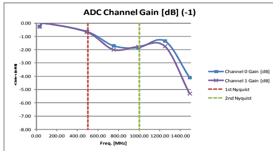
(a) ADC normalized gain vs. frequency (AC version)
