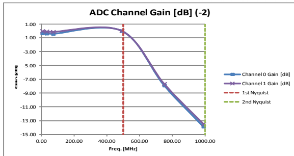
(c) ADC normalized gain vs frequency (DC version)
