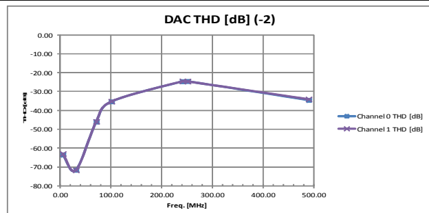
(h) DAC THD vs frequency (DC version)
