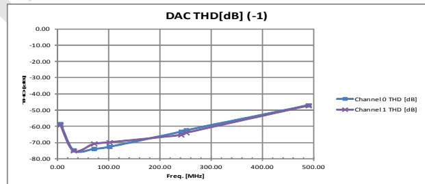
(f) DAC THD vs frequency (AC version)
