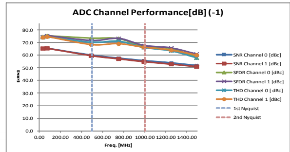
(b) ADC SNR/SFDR/THD vs frequency (AC version)
