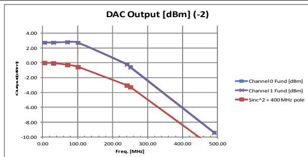
(g) DAC normalized gain vs frequency (DC version)
