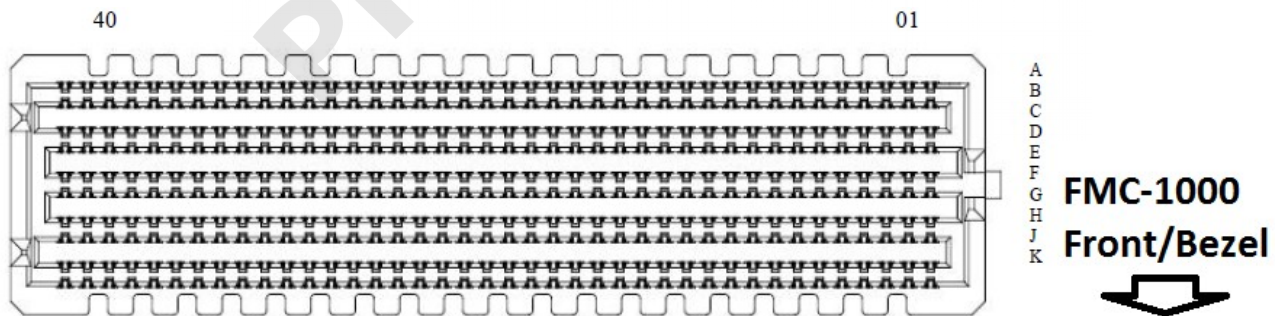
FMC Connector Grid (Component side)
